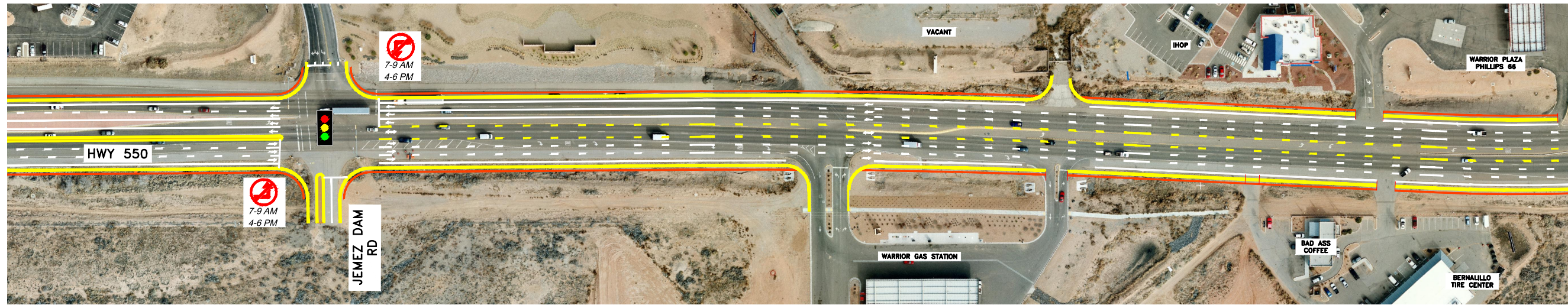
Reversible Lane
